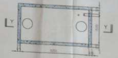
PLAN OF 1000 GLS. CAPACITY SEMI-DIAPHRAGM WATER RESERVOIR SCALE: 1/50
